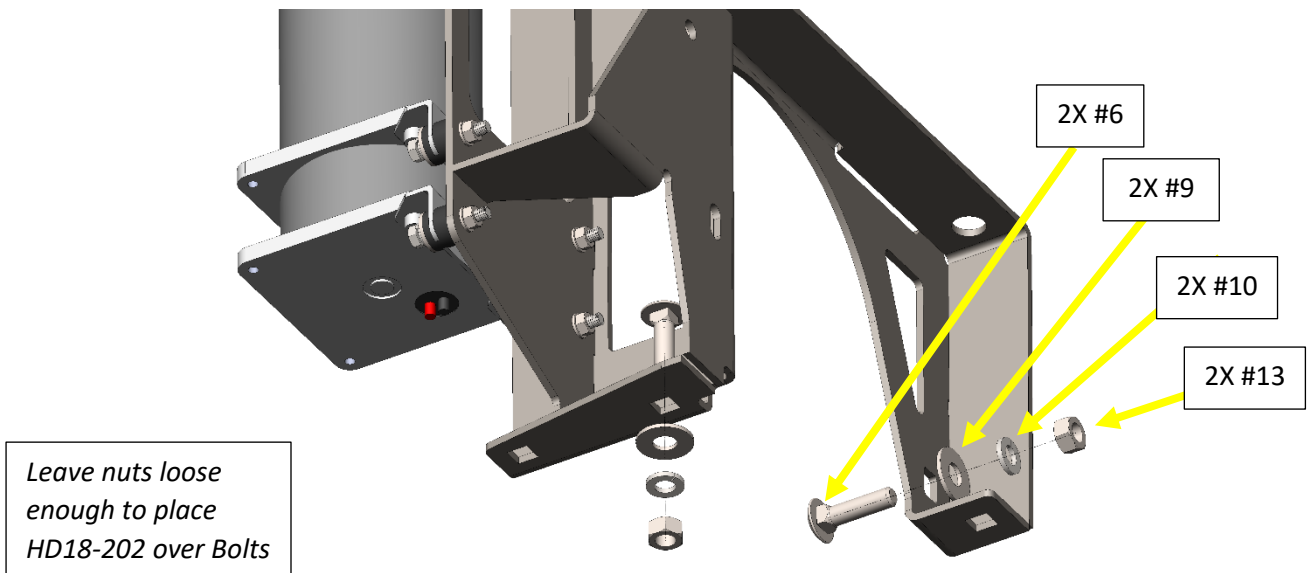
Figure 9 - HD18-101 Bracket with HD18-202 attachment bolts, exploded view
