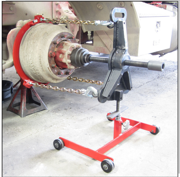
K-1356 Brake Drum Puller shown with K-1350 Wheel Grabber
