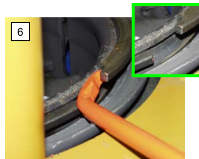
6 Raise the ring until it stays in place.
