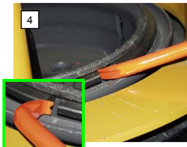
4 Once the rings are parted, insert the "claws" of the PRY-OUT end behind the slotted end of the split ring.
