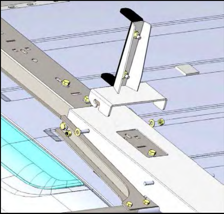
Rear bow location for step ladder.
