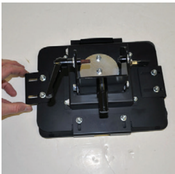
Move all adjustments on Mounting Station to make a snug fit onto tablet.
