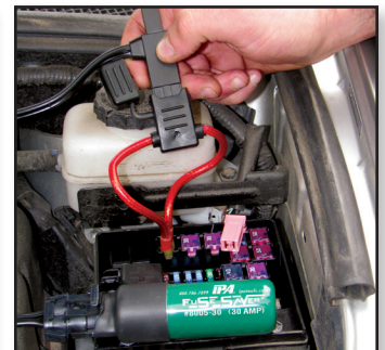
The Fuse Saver® Master Kit Provides a Level of Versatility in Electronic Testing Never Before Available
