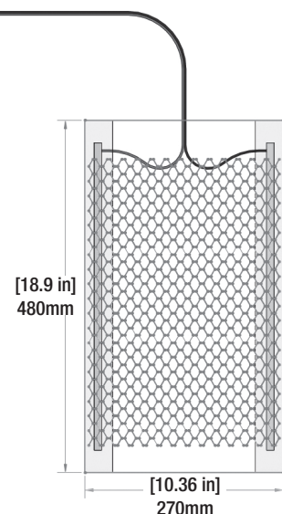
Carbon Fiber Heating Element (IBHS1-XL)
