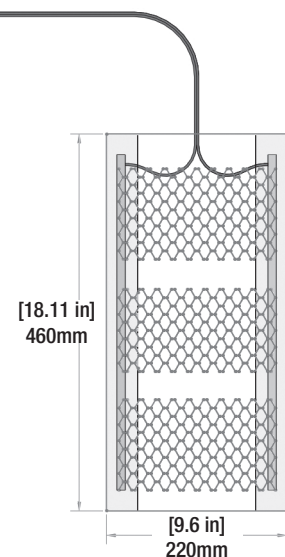
Carbon Fiber Heating Element (IBHS1, IBHS2 & IBHS3)
