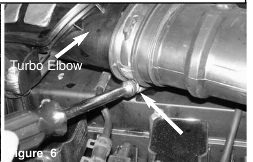
Figure 6 Loosen the clamp on the plastic turbo elbow. Remove the stock intake tube from the turbo elbow.
