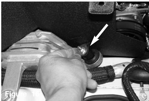
Figure 16 Mount the lower heat shield bracket onto the stand off stud from figure 10. Then place a washer and a M6 nut onto the stand off.
