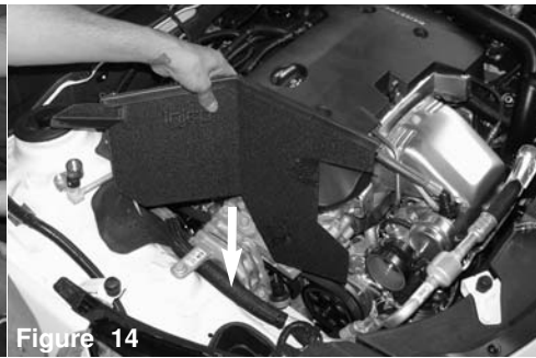
Figure 14 Position the heat shield into the engine bay.
