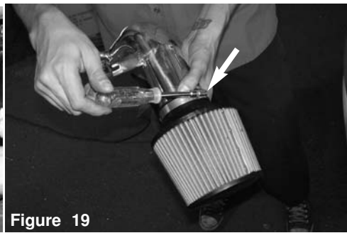
Figure 19 Place the filter onto the bracket side of the intake pipe and then secure the clamp with a 8mm nut driver.
