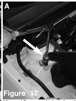
Figure 17 Use a 10mm socket and ratchet and secure the two M6 nuts on the upper left and lower heat shield brackets in figure A and B.
