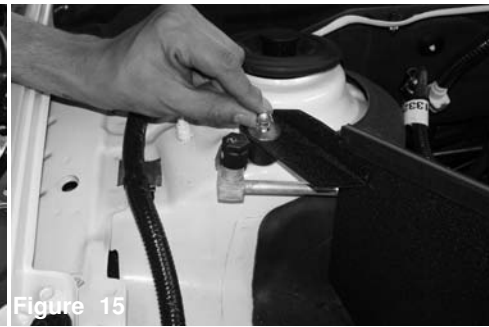
Figure 15 Mount the upper left heat shield bracket onto the male/female vibramount on the shock tower. Place a washer and M6 nut onto the bracket.
