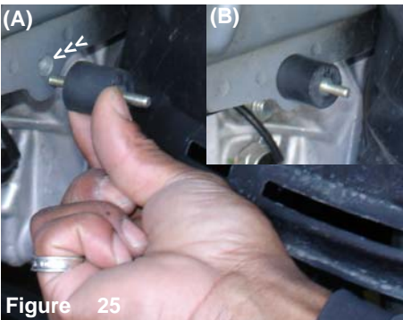
Figure 25 Align the m6 vibra-mount to the pre-tapped hole located on the frame (A). Turn the vibra-mount until the vibra-mount sits flush with the frame (B).
