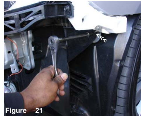
Figure 21 The first m6 bolt is removed from the splash guard.
