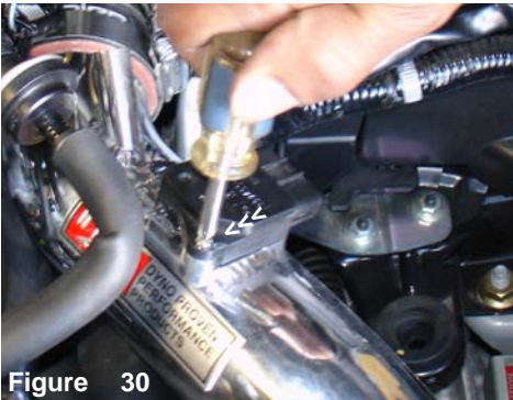
Figure 30 Once you have pressed the mass air flow sensor into the sensor adapter, use the stock screws to secure the sensor to the adapter.
