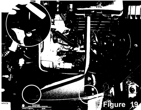
Now install the heat shield and position the tabs on heatshield to the factory ram scoop from step 11. Secure using factory screws. Tighten the rear tab using provided M6 allen screw and fender washer.
