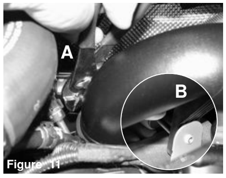
Figure 11 A) With pliers, pinch the clamp holding in intake tube at the turbo. B) With T30 torx bit, loosen and remove the screw holding in intake tube near fire-wall on engine.
