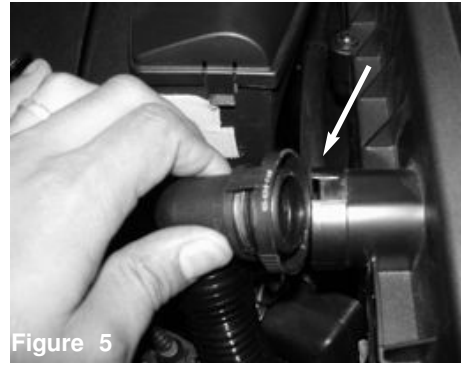
Figure 5 Pinch the harness on smog pump and pull away from air box. (if equipped with smog pump)
