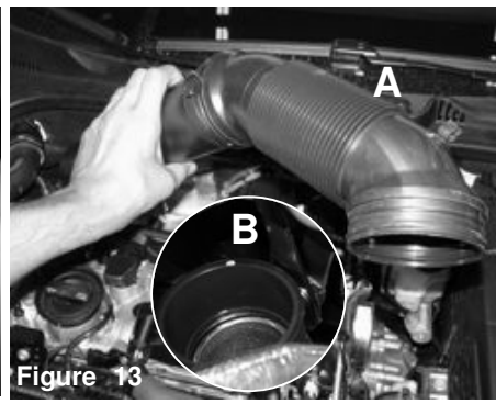
Figure 13 A) Remove intake tube out of vehicle. B) Pinch remaining clamp on turbo and remove.
