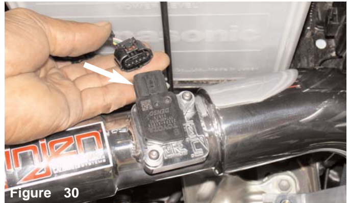
Figure 30 Press the electrical harness clip over the mass air flow sensor until it snaps in place.
