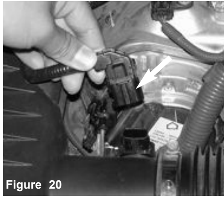
Depress the tab and pull the electrical harness connector from the mass air flow sensor.
