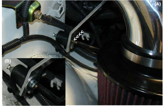
The intake bracket is aligned to the vibra-mount stud (A). Use the m6 flange nut and fender washer to secure the intake in place (B).
