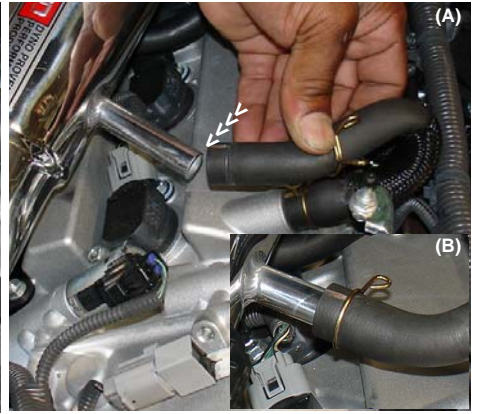
Take the stock breather hose and press it over the 5/8" intake port (A), the tension clamp is used to secure the hose over the intake port (B).
