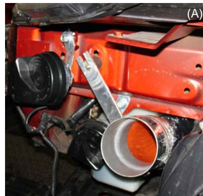
Once the coupler has been pressed into the silicone hose, align the coupler bracket to the vibra-mount stud (A). Place the fender washer and m6 flange nut over the vibra-mount stud and use the 10mm socket to fasten the flange nut to the vibra-mount stud (B).
