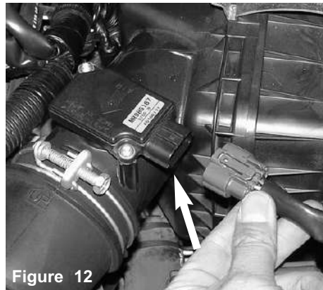
Figure 12 Depress the clip on top of the harness and pull the harness away from the mass air flow sensor.
