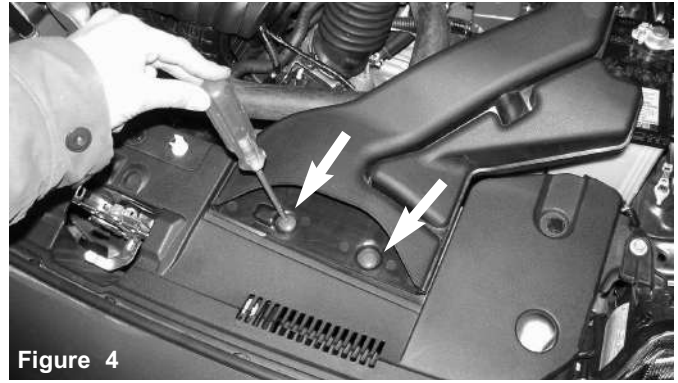
Figure 4 A phillips screw driver is used to loosen the two plastic clips.
