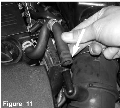
Figure 11 Once the tension clamp as been pulled back, pull the crankcase vacuum hose from the air duct port.
