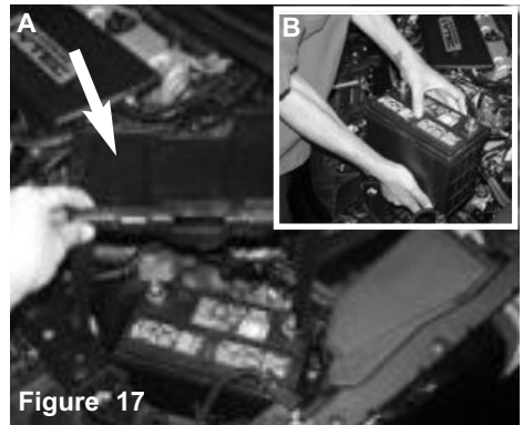
Figure 17 Figure A: Remove the battery cover. Figure B: Now remove the battery from the engine bay.
