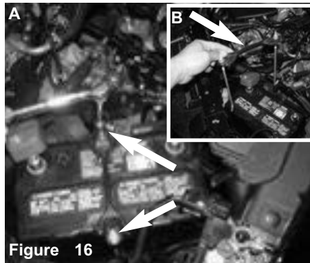
Figure 16 Figure A: Loosen the 10mm nuts on the battery tie down. Figure B: Unhook the battery tie down hooks from the frame and then remove from engine bay.,
