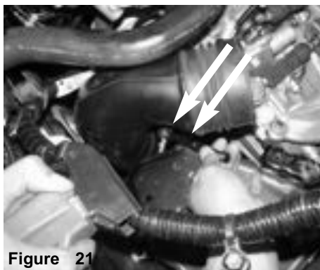
Figure 21 Remove the two 10mm bolts attaching the lower air box resonator duct to the battery support bracket.
