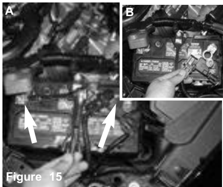
Figure 15 Figure A: Loosen the 10mm nuts on the positive and negative battery terminals. Figure B: Detach both battery terminals from the battery.
