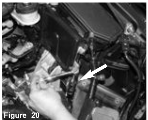
Figure 20 Use a 10mm socket and ratchet and remove the 10mm bolt connecting the ECU bracket to the battery support bracket.
