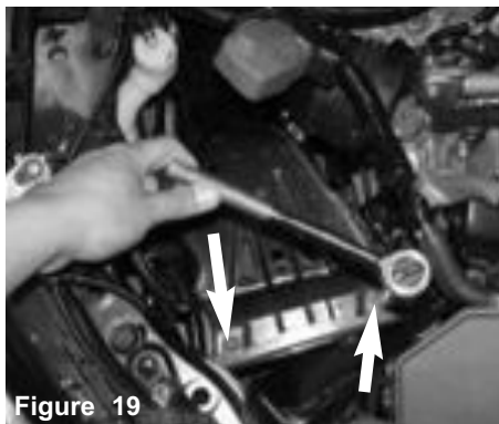
Figure 19 Use a 12mm socket and ratchet and remove the two 12mm bolts on the battery support bracket attached to the chassis
