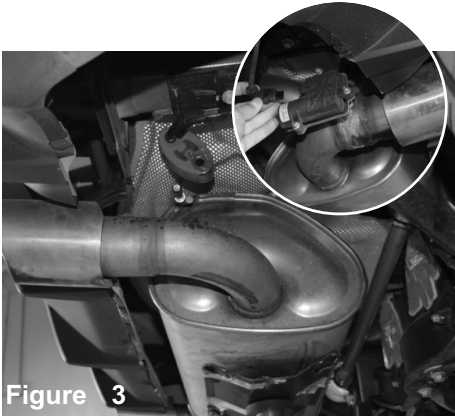
Figure 3 Lubricate all hanger isolators and pull back. Disconnect the Exhaust Valve sensor harness.
