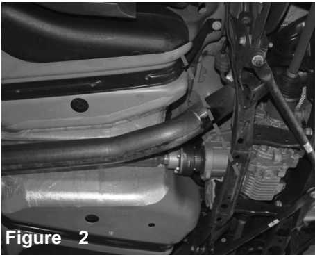
Figure 2 Locate this spot on the factory exhaust, this is a great spot to cut and also, if needed to re-install, you can have welded to have stock exhaust installed.
