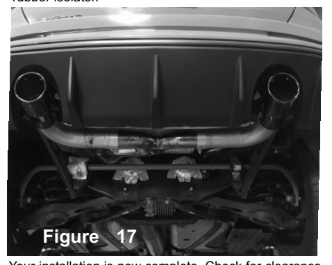
Figure 17 Your installation is now complete. Check for clearance and position for best possible fit. Re-install the mid-frame support brace. Make sure there is clearance and the exhaust is not touching.
