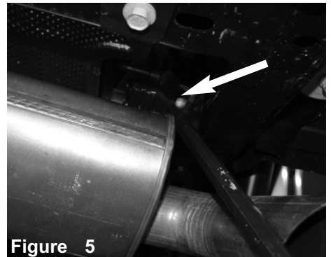
With lubrication, pull back the rubber hangars from exhaust.
