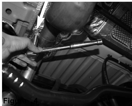
Loosen the 15mm nut on OEM clamp. Loosen and pull back.
