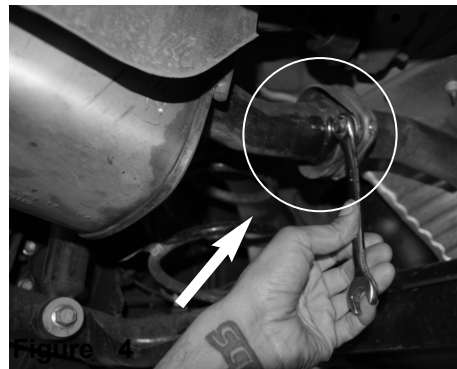
Loosen and remove the rear section of the exhaust using 14m socket or wrench.
