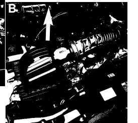
Figure 7: Use a 8mm nut driver and loosen the clamp on the throttle body. Figure 8: Firmly lift up on the air box assembly and remove the entire air box assembly and air duct.
