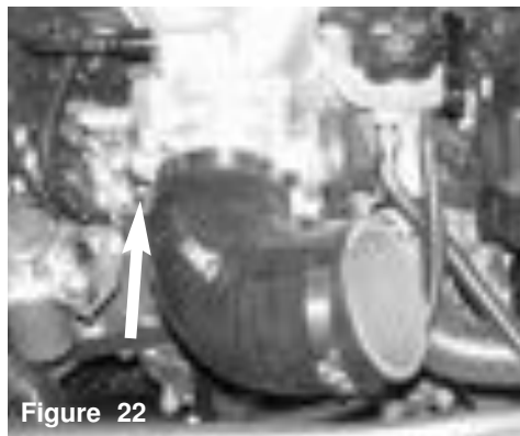
Figure 22 The 90 degree elbow is now resting over the throttle body, the clamp over the throttle body is semi-tightened.
