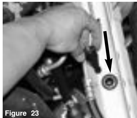
Figure 23 The Injen stand-off is lined up to the stock grommet.
