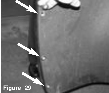
There are four plastic clips that need to be removed from the mud flap. There are three clips to the outside and one clip to the inside of the mud guard.
