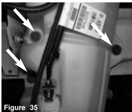
Loosen and remove all three m6 bolts securing the reservoir bottle to the frame.
