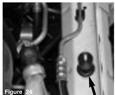
Figure 24 The stand-off is firmly pressed into the grommet as shown above.
