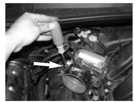
Figure 10 Secure the clamp on the throttle body for now.
