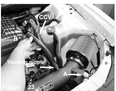
Figure 23: (A) Use a M6 nut and fender washer to secure the intake bracket to the vibramount. Make your final adjustment and secure the clamp on the hose in figure 5 (B) Use the 10"-15mm vacuum hose and connect the vacuum nipple on the intake tube to the crank case vent tube
