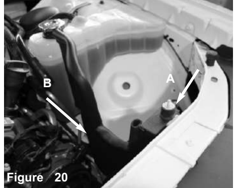
Figure 20: (A) Once the heatshield is aligned, place a vibramount onto the front heatshield bracket to secure it to the bracket on the front radiator support. (B) Use a M6 nut to secure the back of heatshield to the vibramount from figure 16.
