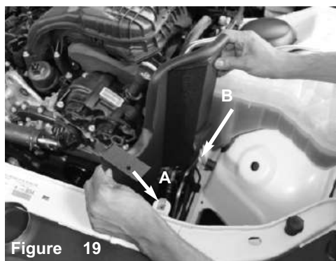
Figure 19: (A) Align the front heatshield tab to the bracket on the front radiator support. A vibramount will be used to secure them together in the next step. (B) Align the hole in the back of the heatshield to the vibramount from figure 16.
