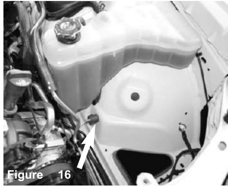
Figure 16: Place a vibramount on the pre-drilled hole on the inner wheel well in the engine bay. You will have to secure the vibra mount from the outer wheel well using a supplied M6 nut. Figure 17 will illustrate how
