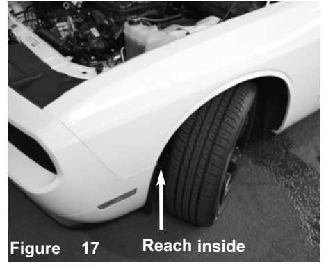
Figure 17 Turn the steering wheel to the left. This will give you access to the outer wheel well to secure the M6 nut to the vibramount from figure 16. No wrench necessary, just turn the vibramount until it's snug.
