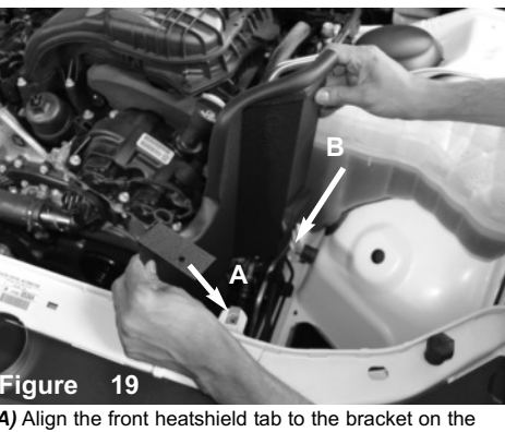
Figure 19 (A) Align the front heatshield tab to the bracket on the front radiator support. A vibramount will be used to secure them together in the next step. (B) Align the hole in the back of the heatshield to the vibramount from figure 16.
