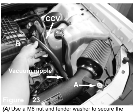
Figure 23 (A) Use a M6 nut and fender washer to secure the intake bracket to the vibramount. Make your final adjustment and secure the clamp on the hose in figure 5 (B) Use the 10"-15mm vacuum hose and connect the vacuum nipple on the intake tube to the crank case vent tube
