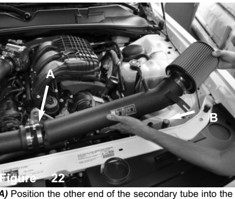
Figure 22 (A) Position the other end of the secondary tube into the primary tube from figure 15 (B) Also, Align the Bracket on the secondary tube to the vibramount on the radiator support from figure 20.
