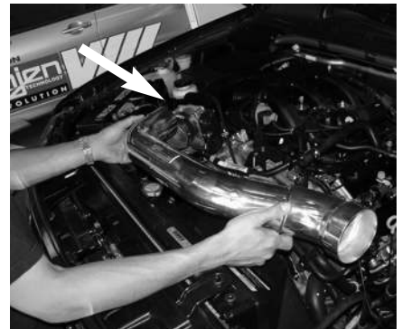
Lower the Injen intake pipe into the engine bay and place the 2.75" pipe end into the 2.75" straight hose already on the throttlebody.
