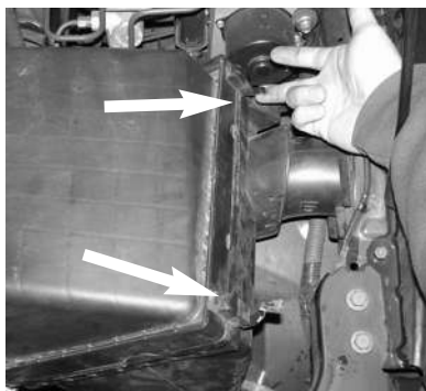
Unclip two retaining tabs holding the upper part of the air box to the lower part of the air box
