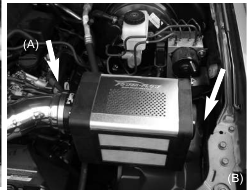
The four inch velocity stack base is connected to the intake (A) and the Power box bracket is lined up to the vibra-mount stud (B).
