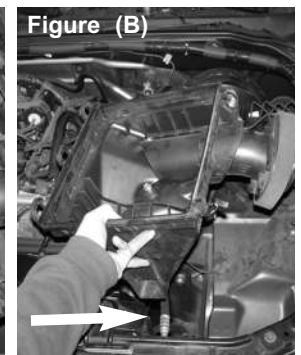
Remove 10mm bolt located on the right upper portion of the air box (Figure A). Lift air box up and off the lower grommet located at the bottom of the air box. Stock air box component removal is now complete.
