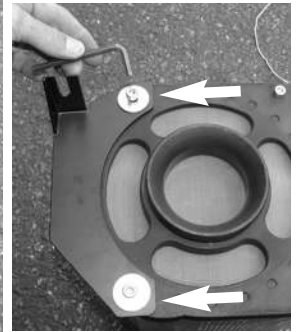
Reuse the 45mm bolts and use two supplied fender washers to mount the bracket onto the box.
