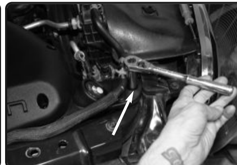
23. Use the M8X40 bolt to secure the air box bracket to the radiator support
