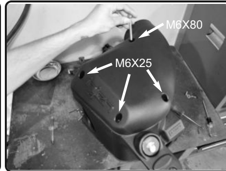
15. Place the plenum onto the lower air box and place 1-M6X80 and 3-M6X25 as illustrated in the photo.
