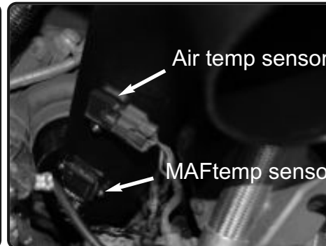
19. Once the tube is in place, re-connect the MAF and air temp sensor on the intake tube
