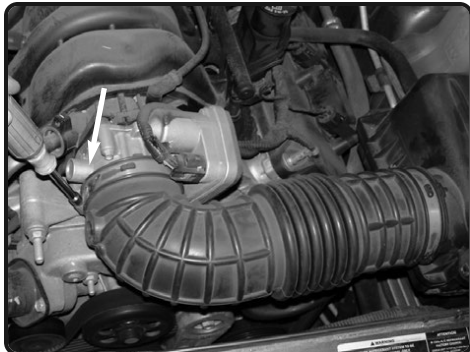
5. Loosen the clamps on the air box and throttle body using 8mm nut driver.
