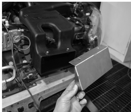
Install the rain guard. Secure using provided M6 socket cap screws and tighten.
