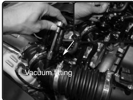
7. With 10mm socket, remove the 2 screws holding in vacuum fitting. Carefully pull back fitting.
