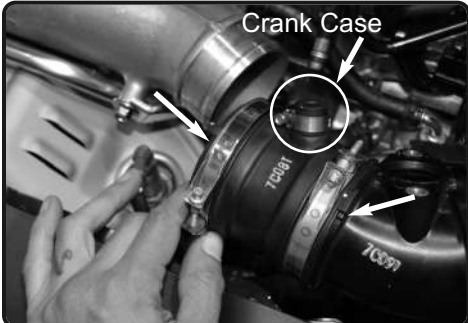
9. Now pull back the intake tube from turbo. Brake the crank case clamp using pliers to remove. Remove the crank case hardline out of intake tube.
