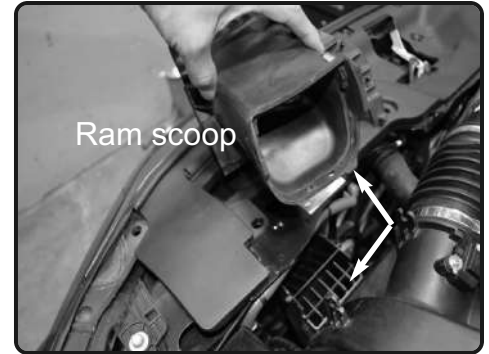
4. Now lift up and pull back the Rubber ram scoop. Note: there are plastic fittings holding in scoop, pull rubber away from fittings.
