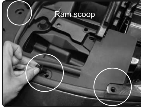
3. Carefully remove the push-clips from the upper engine cover.
