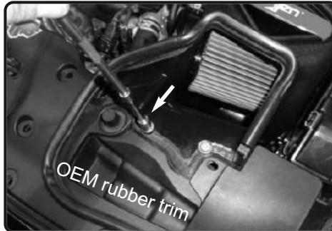
23. Re-install shroud, secure the front of the air box to the vehicle using originals screws from step 2. install the remaining rubber trim to the shroud.
