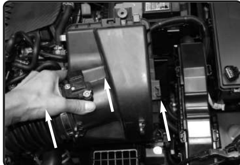
10. Lift up and remove the airbox.
