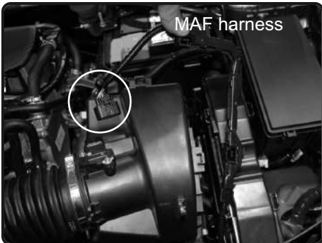
5. Disconnect the MAF sensor harness. Pull back the line away from the airbox.
