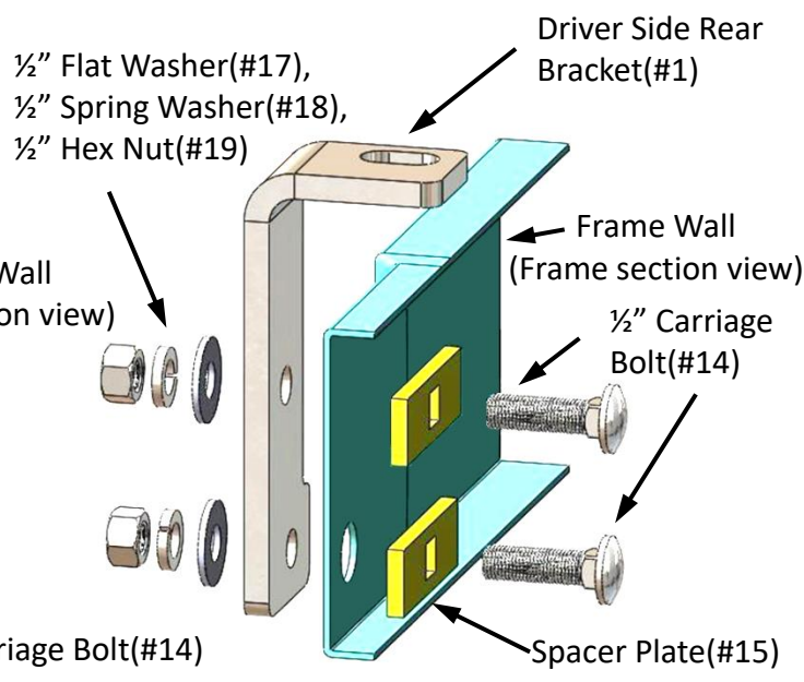
Driver Side Rear Bracket Shown
