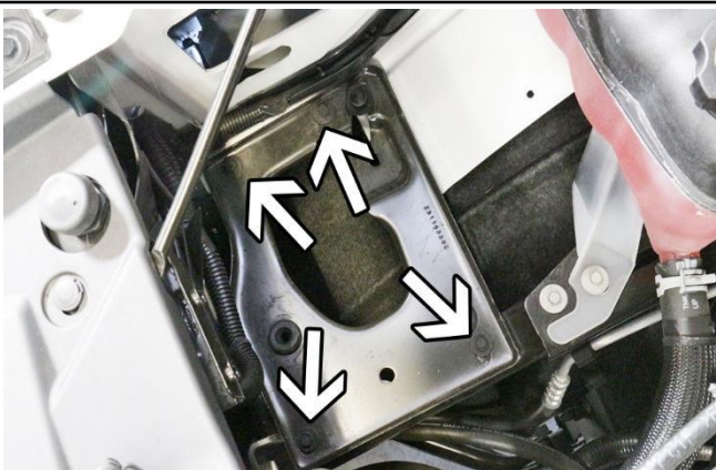
10. Remove the four bolts securing the air box mounting tray and remove the tray from the vehicle.
