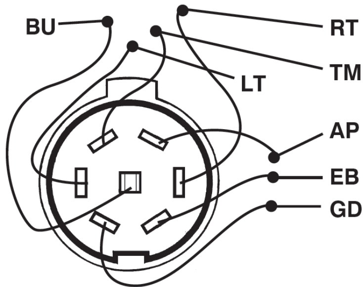
VIEW LOOKING AT FRONT OF PLUG
