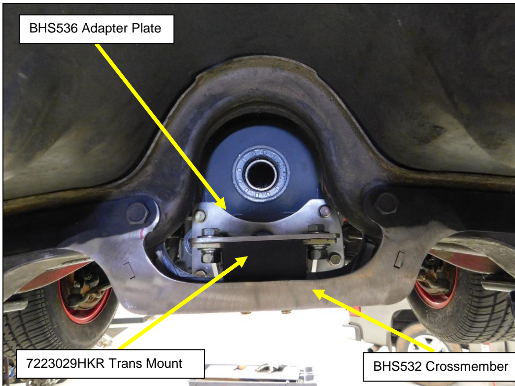
Shown with 8HP70 Transmission Installed
