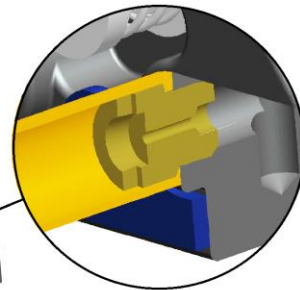
CROSS-SECTION OF JET INSTALLED INSIDE EXTENSION
