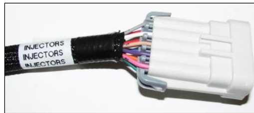
Figure 22 Fuel Injectors
