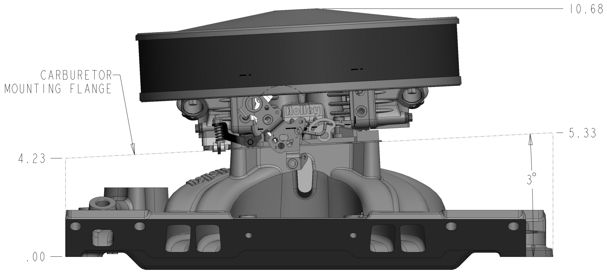
300-264 SHOWN WITH 4150 CARBURETOR AND 120-102 14" AIR CLEANER
