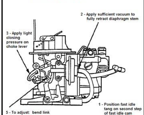
FIG. 9 - CHOKE QUALIFYING
