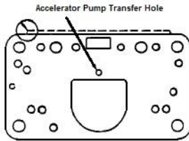
METERING BODY GASKETS
