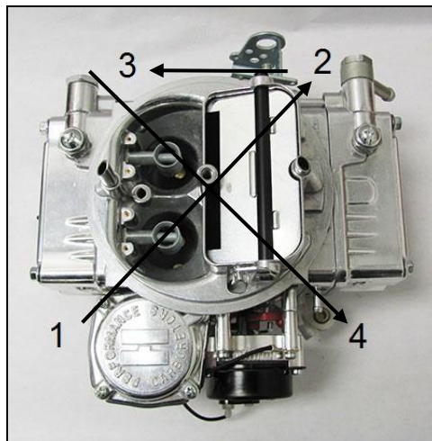
Figure 1—Carburetor torque sequence (all Holley® carburetors)
