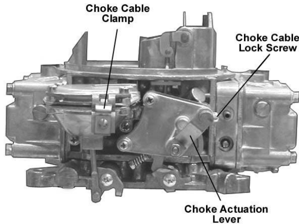
Figure 2b. Manual choke parts (0-1850 shown)
