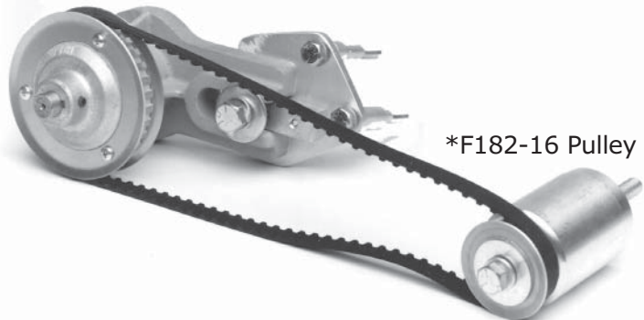
*PDC-6 Timing Belt Drive (This combination drives the fuel pump at 1/2 engine speed)
