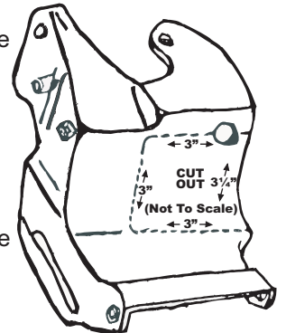
Power Steering Pump Mounting Brackets:
