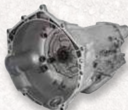
19260380 Hydra-Matic 4L65-E Four-Speed Automatic Transmission Electronically controlled four-speed over-drive transmission. Suitable for engines producing up to 430 lb.-ft. of torque.
