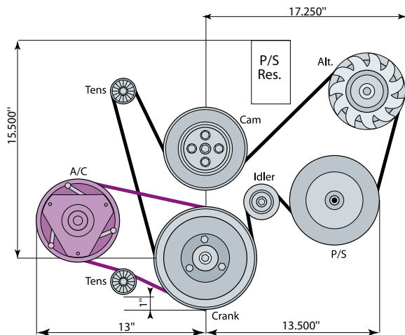
Corvette Accessory Drive System, with A/C E
