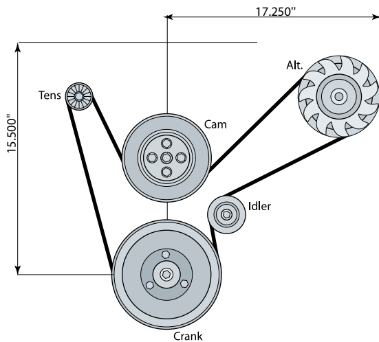
DR525 Accessory Drive System C
