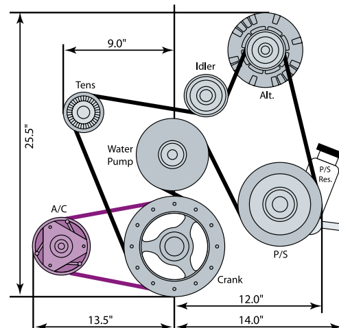
LC9 5.3L Accessory Drive System (19258433) with LC9 5.3L A/C Add-on Kit (19260892)
