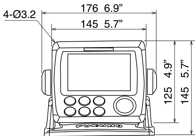
GP33 Display Unit (Bracket Mount)
