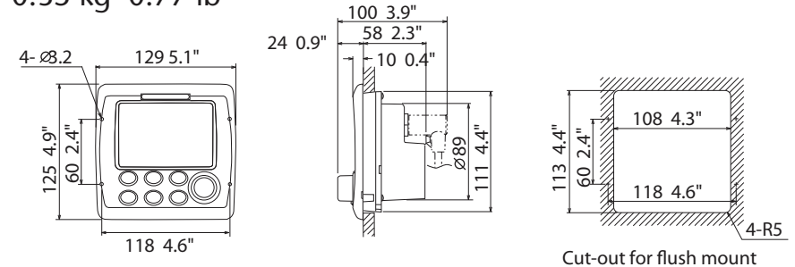
NAVpilot-711 Control Unit (Flush-mount) 0.35 kg 0.77 lb
