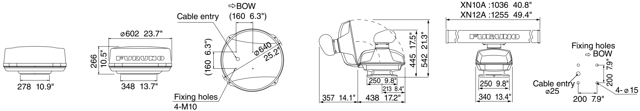
24" Radome Antenna
