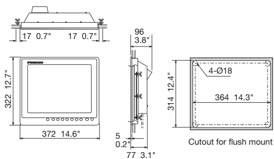
MU150HD Flush Mount
