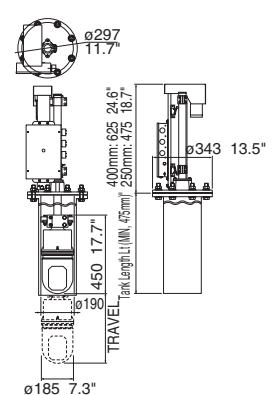
CH300 (Hull Unit) CSH304 (Travel: 400 mm) 43 kg 94.8 lb CSH305 (Travel: 250 mm) 42 kg 92.6 lb
