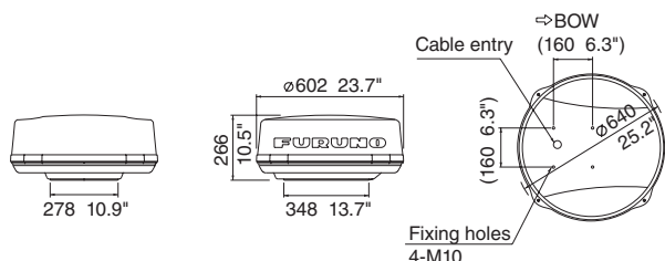
24" Radome Antenna
