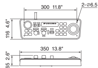
CSH5211-A Control Unit 3.5 kg 7.7 lb
