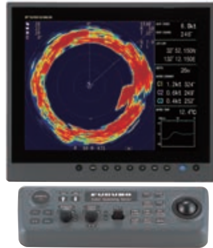
FULL-CIRCLE SCANNING SONAR Model CSH8L MARK-2
