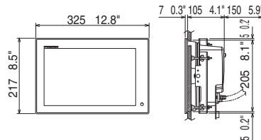
Multi Function Display (Flush Mount) TZTL15F
