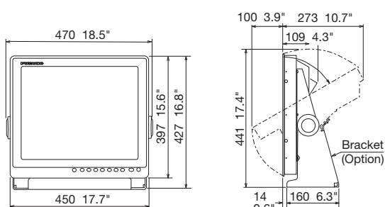
MU190HD Bracket Mount
