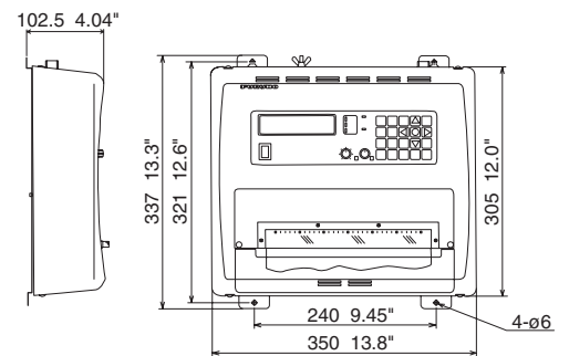
FAX408 Receiver Unit 5.6 kg 12.3 lb
