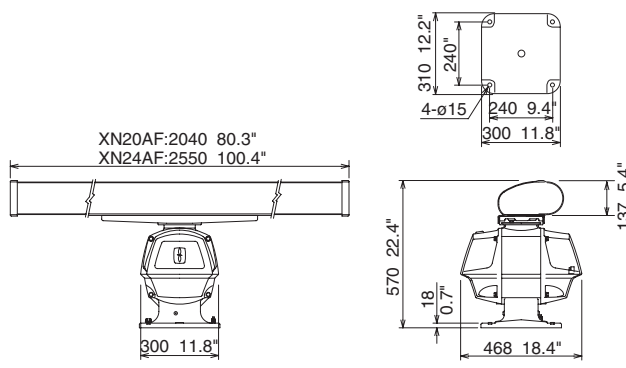
6.5 ft Open Antenna 8 ft Open Antenna
