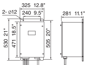
CSH5130-A-5L Transceiver Unit 20 kg 44.1 lb
