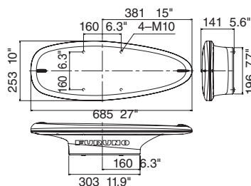
SC50 Antenna Unit (Open)
