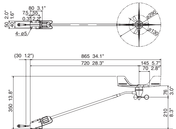
Wind Transducer FI5001L (Long Shaft)
