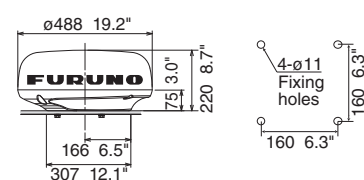
MODEL1815 Antenna 6.5 kg 14.3 lb
