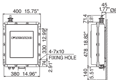
Antenna Coupler AT5075 9.2 kg 20.1 lb
