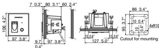
Remote Control Unit MCU-004 (option)
