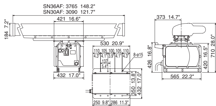
12 ft S-band Antenna SN30AF 14 ft S-band Antenna SN36AF
