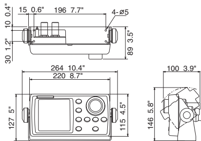
NAVipilot 700 Control Unit (Bracket Mount)
