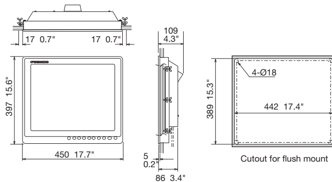
MU190HD Flush Mount
