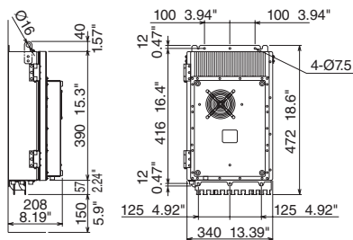
Transceiver Unit FS1575T 16 kg 35.2 lb
