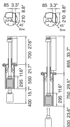
CSH5040-A (600 mm travel) Hull Unit 75 kg 165 lb CSH5041-A (400 mm travel) Hull Unit 70 kg 154 lb
