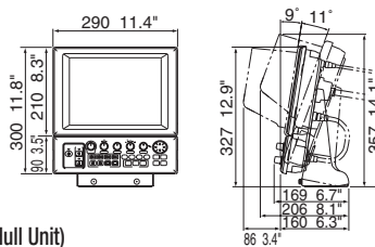
CH250 (Hull Unit) CSH254 (Travel: 400 mm) 43 kg 94.8 lb CSH255 (Travel: 250 mm) 42 kg 92.6 lb
