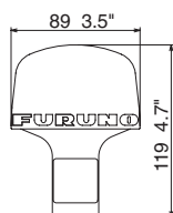
GPS/WAAS Receiver Antenna BBWGPS 10 m cable attached
