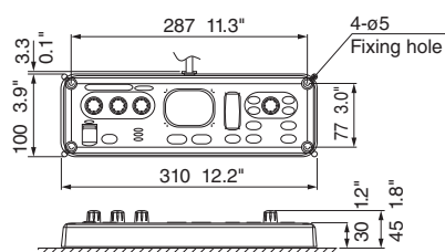
FAR1518/1528 Control Unit
