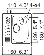
Trackball Control Unit RCU-015
