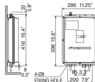
Antenna Coupler AT1575-AES 2.6 kg 5.7 lb
