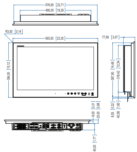
MU240T (Flush Mount)
