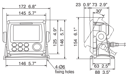
GP39 Display Unit (Bracket Mount)
