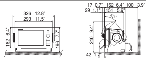
Multi Function Display (Tabletop Mount) TZT9 4.7 kg 10.4 lb
