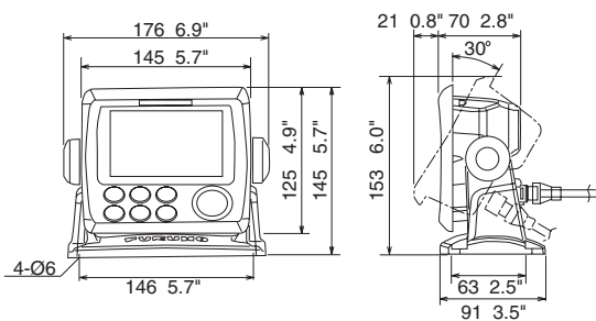
RD33 Display Unit (Bracket Mount)
