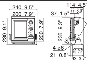
MODEL1815 Display Unit (Bracket Mount) 2.2 kg 4.9 lb
