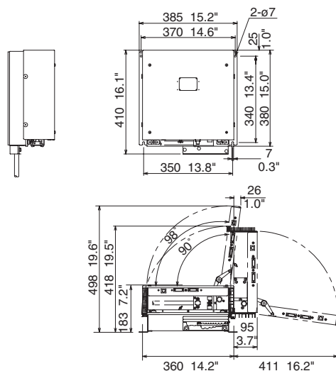
Processor Unit RPU-013
