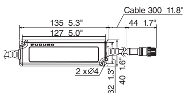
Analog NMEA Data Converter IF-NMEAFI (option)
