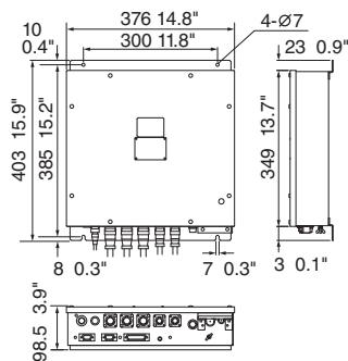
CSH5210-A Processor Unit 3.4 kg 7.5 lb
