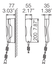
Handset HS2003 0.5 kg 1.2 lb
