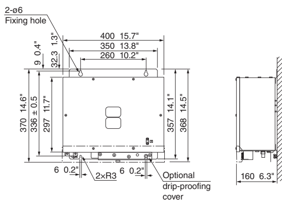
FAR1518/1528 Processor Unit
