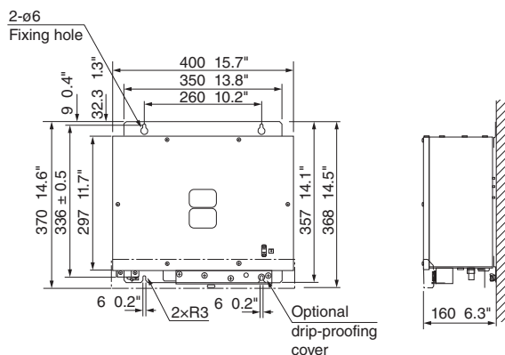
FAR1513/1523 Processor Unit
