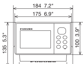
GP39 Display Unit (Bracket Mount)
