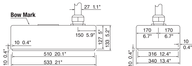
WMB5230 80 kHz TRANSDUCER
