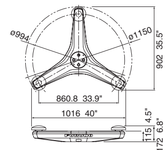
SC110 Antenna Unit
