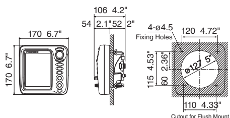
FCV628 (Flush Mount)
