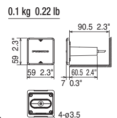
SD Card Unit SDU-001 (option)
