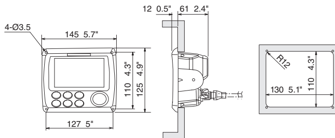
RD33 Display Unit (Flush Mount)
