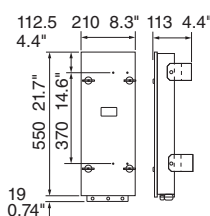
CSH5020-A Preampifier 6.5 kg 14.3 lb
