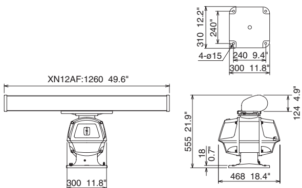
4 ft Open Antenna
