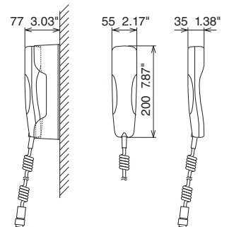
Handset HS-2003
