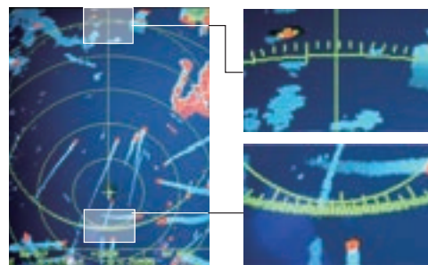
Clearance between markings of the bearing scale is changed according to the proximity between own ship and the bearing circle, as shown in the images on the left-hand side. It helps to grasp the bearing to the target echo without using an EBL.
