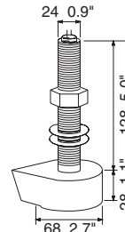
Transducer Bronze 520-5MSD (Metal, Thru-hull)
