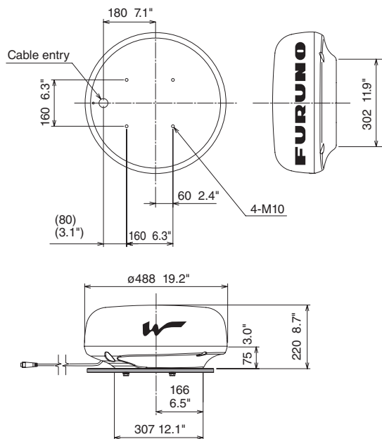
1st Watch Wireless Radar DRS4W
