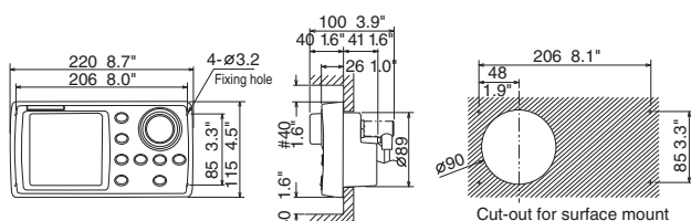
NAVipilot 700 Control Unit (Surface Mount)
