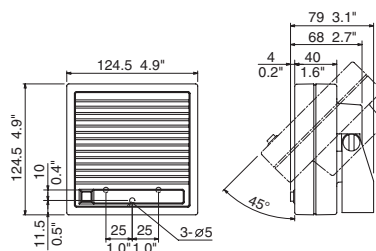
NX300 Display Unit
