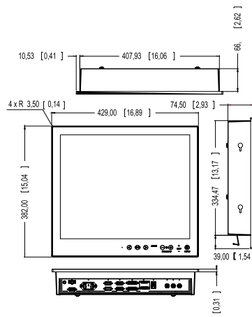
MU190T (Flush Mount)
