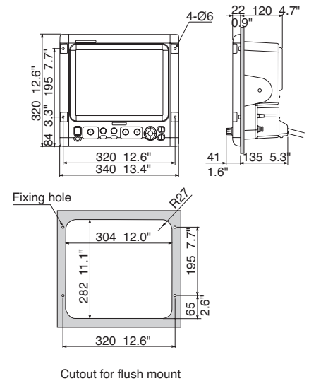
FCV1150 (Flush Mount)
