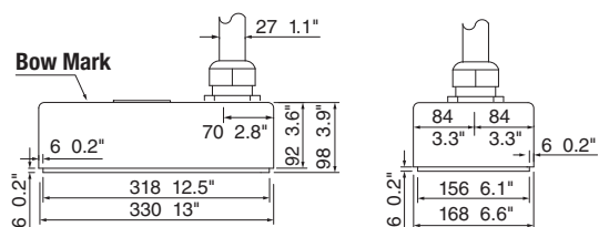
WMB3230 160 kHz TRANSDUCER
