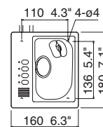
Remote Control Unit RCU-016
