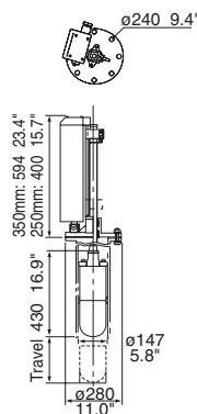
CH270 (Hull Unit) CSH181 (Travel: 350 mm) 37 kg 81.6 lb CSH184 (Travel: 250 mm) 35 kg 77.2 lb
