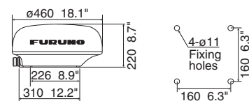
MODEL1715 Antenna 5.1 kg 11.2 lb
