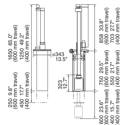
CSH8040-A (600 mm travel) Hull Unit 82 kg 180.8 lb CSH8041-A (400 mm travel) Hull Unit 81 kg 178.6 lb
