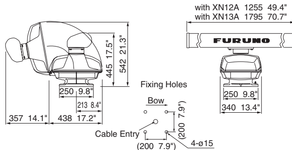
6 ft Open Antenna
