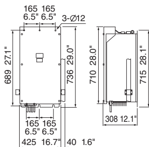
CSH8030-A-8L Transceiver Unit 37 kg 81.6 lb
