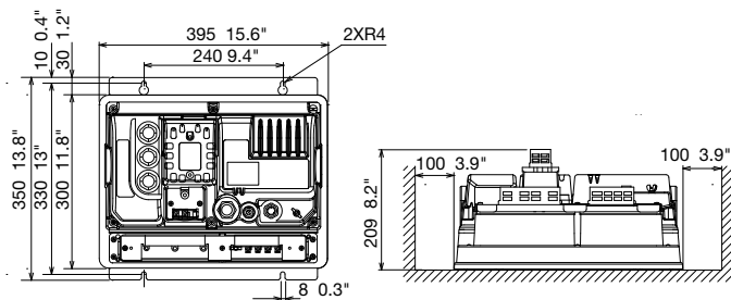
Remote Control Unit MCU-002 (option)
