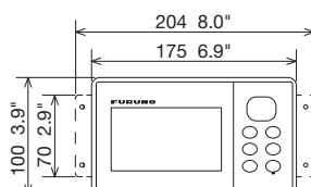
GP39 Display Unit (Flush Mount)
