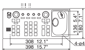
Full-keyboard Control Unit RCU-014
