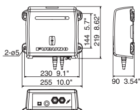
Network Fish Finder DFF1/Bottom Discrimination Sounder BBDS1 1.3 kg 2.9 lb
