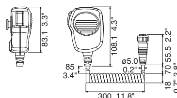
Intercom Speaker LH3010
