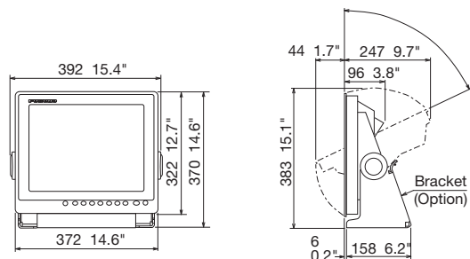
MU150HD Bracket Mount
