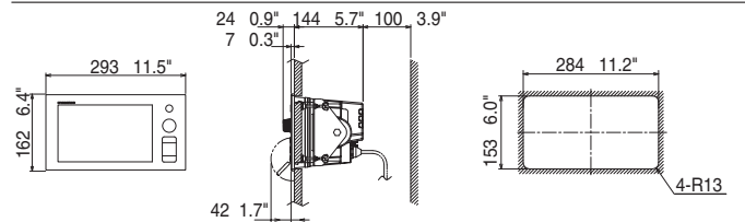
Multi Function Display (Flush Mount) TZT9 4.5 kg 9.9 lb
