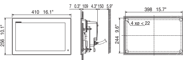
Multi Function Display (Flush Mount) TZTL15F
