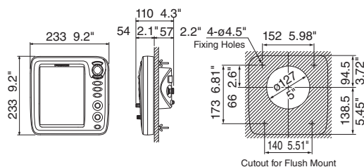
FCV588 (Flush Mount)
