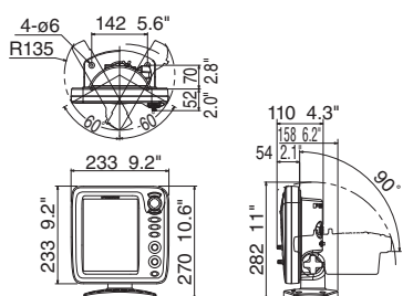
MODEL1815 Display Unit (Bracket Mount) 2.2 kg 4.9 lb
