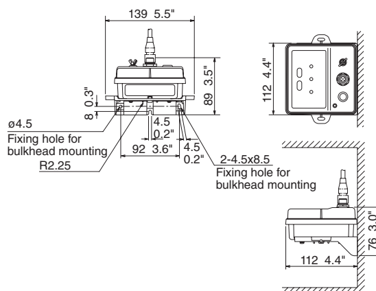
PG700 (bulkhead mounting) Main Unit 0.35 kg 0.77 lb
