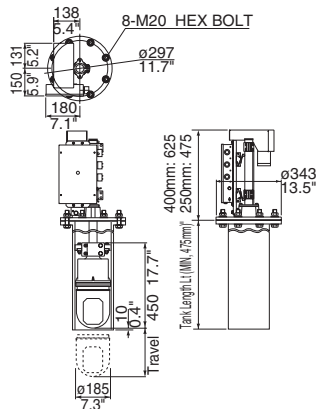
CH250 (Hull Unit) CSH254 (Travel: 400 mm) 43 kg 94.8 lb CSH255 (Travel: 250 mm) 42 kg 92.6 lb
