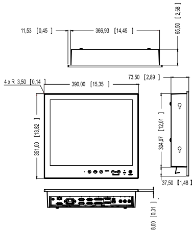
MU170T (Flush Mount)
