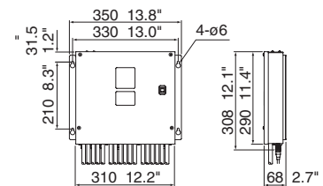
SC50/110 Processor Unit
