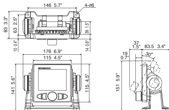
NAVipilot 711C Control Unit (Tabletop Mount)
