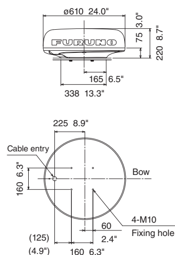
24' Radome Radar Sensor DRS4D-NXT
