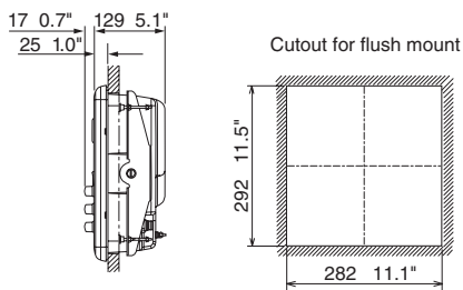
FR8065/8125/8255 Display Unit (Flush Mount)
