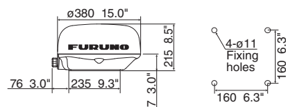
MODEL1715 Antenna 5.1 kg 11.2 lb
