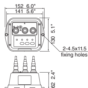
PG500R 0.3 kg 0.7 lb
