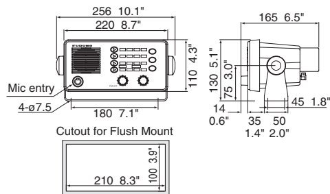
Microphone DM2003
