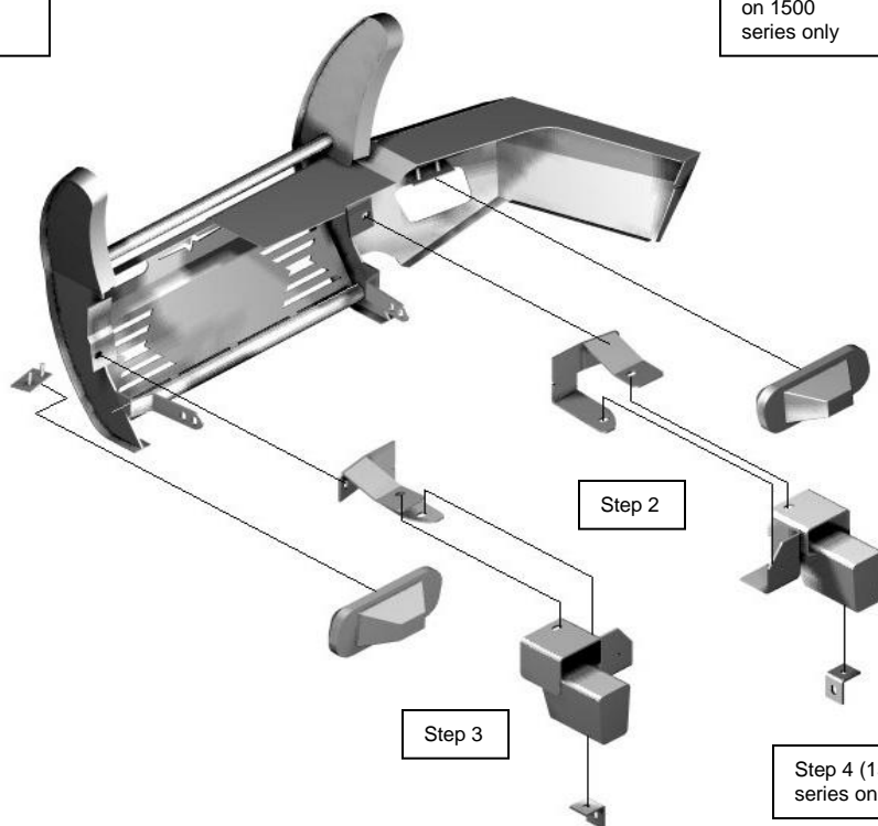
Frame Support Bracket
