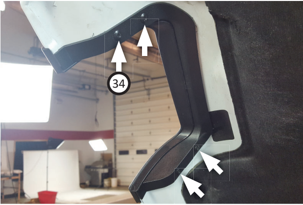
59. Fasten inner hood gasket to hood using (x4) blind rivets (34) through holes drilled in previous step.
