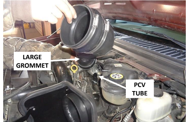
22. Moistening the PCV tube with soapy water will ease its insertion in the next step. Move the intake tube into position for installation, noting the locations of the large grommet and PCV tube.
